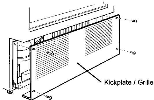
Figure 2-1. Kickplate/Grille Removal
